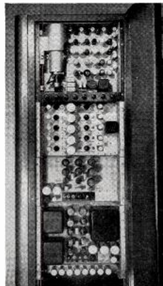
RCA MONOSCOPE television camera (top section of cabinet), distribution amplifier (center) and regulated power supply (bottom) are used to test television equipment in stations and on assembly lines. They are used in conjunction with an RCA synchronizing generator.
